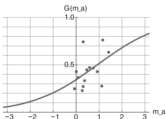
(c) H18 入学—H20 年新司 ( \beta = 0.39, T_A = 0.921 )
